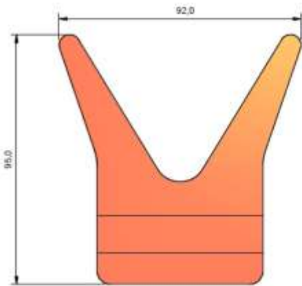
V-BLOCK 18
