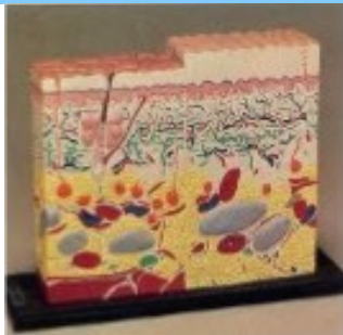
Model human skin
