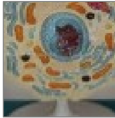
Model animal cell
