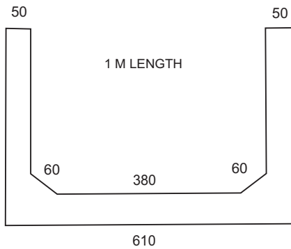
SWC 1 CHANNEL - 180KG
