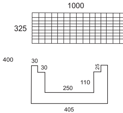
SWC 8 CHANNEL - 80KG
