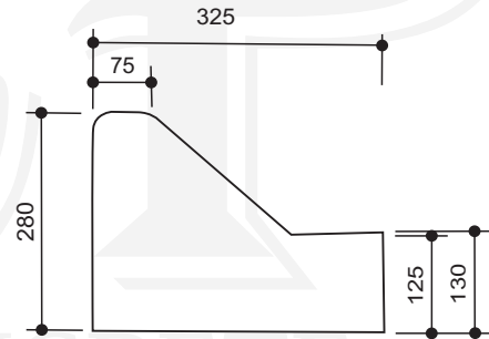
FIG 7 KERB & CHANNEL
