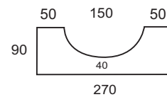
SWC 5 CHANNEL - 55KG
