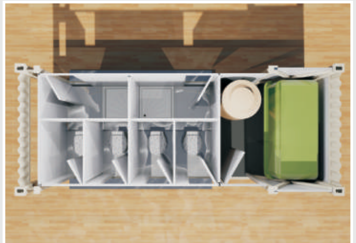
ADVANCED ABLUTION CONTAINER LAYOUT
