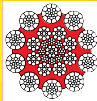
FASTLIFT® Special Wire Ropes
